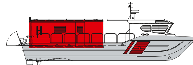
Workboat Lehmar 1500/Steel with 20 ft. Shelter, Medical Care
